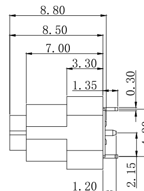
SECTION SCALE 1:1
