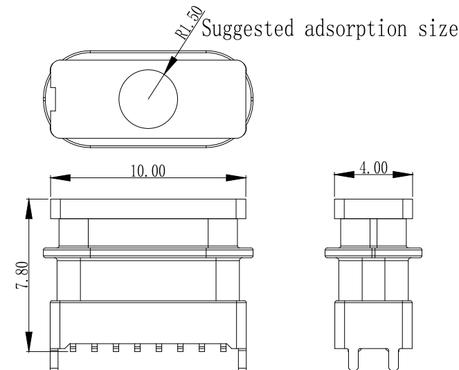
Install suction cap diagram
