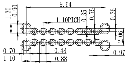
RECOMMENDED P.C.B. LAYOUT TOLERANCE UNSPECIFIED ±0.05mm
